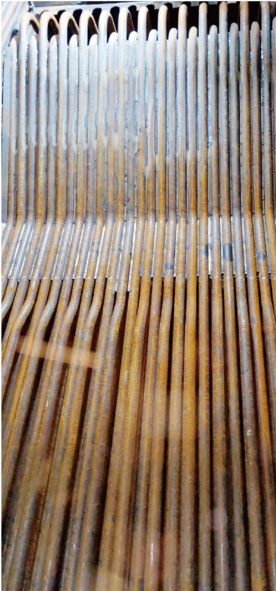
◇ D type boiler retubing
